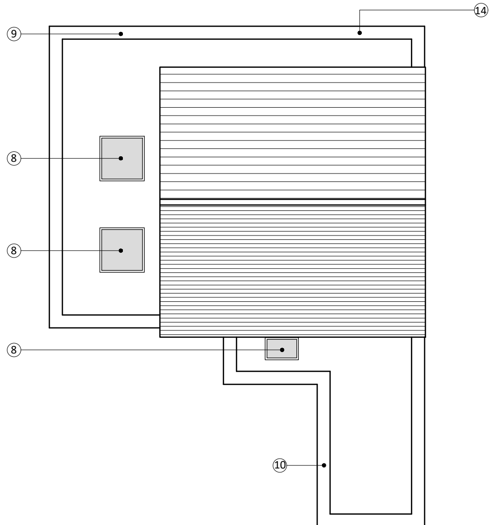
ROOF PLAN
