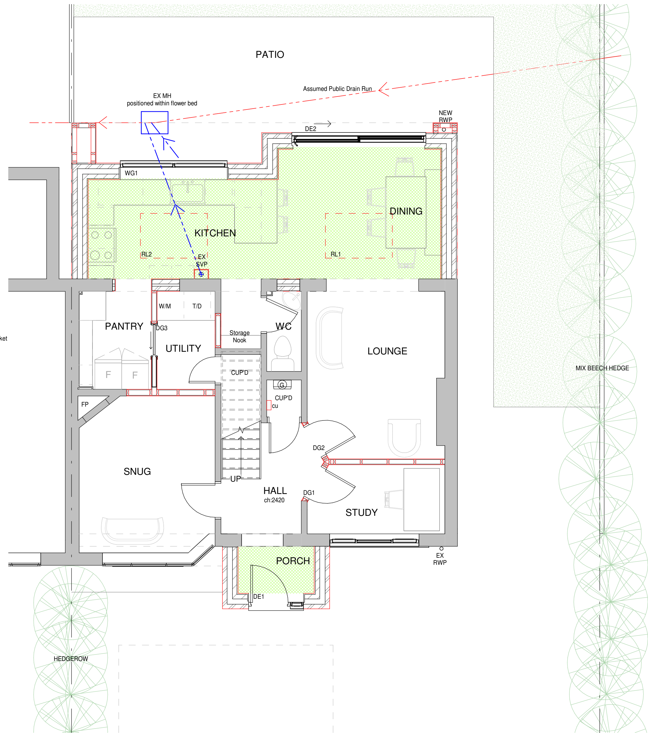
7 Proposed Ground Floor Plan 1 : 50
