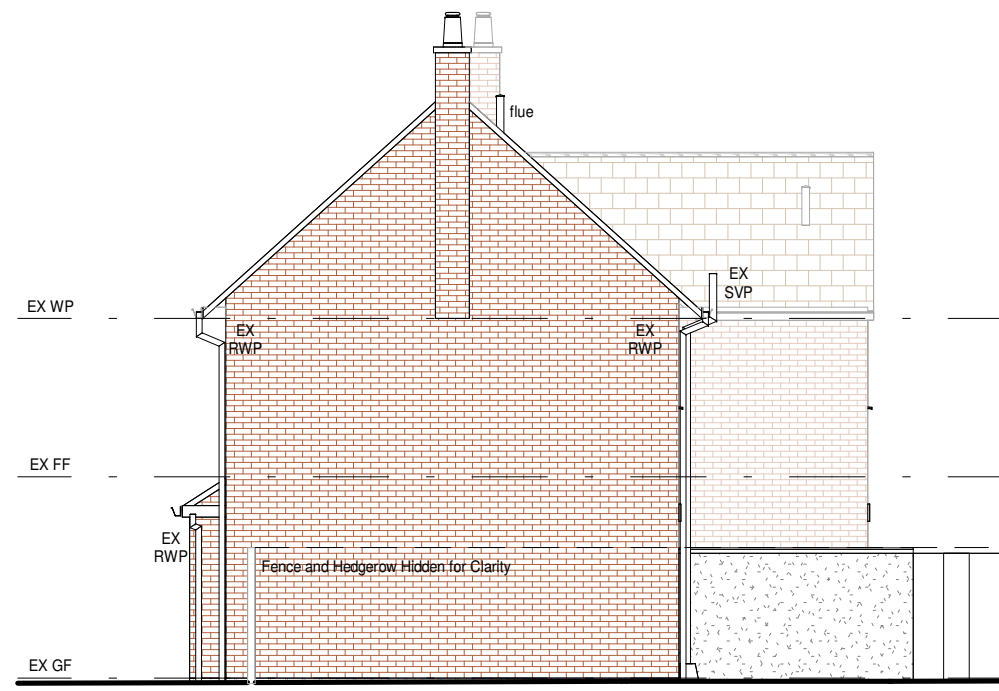
4 Existing North Elevation 1 : 100
