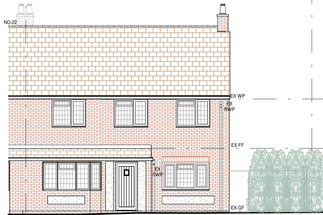
3 Existing East Elevation 1 : 100
