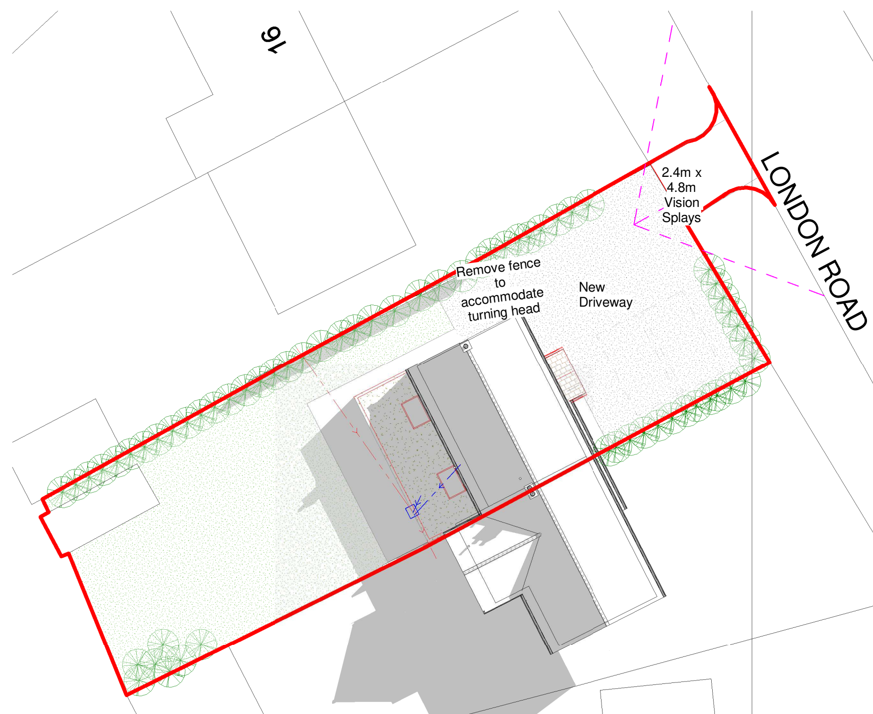
8 Proposed Roof/Site Plan 1 : 200
