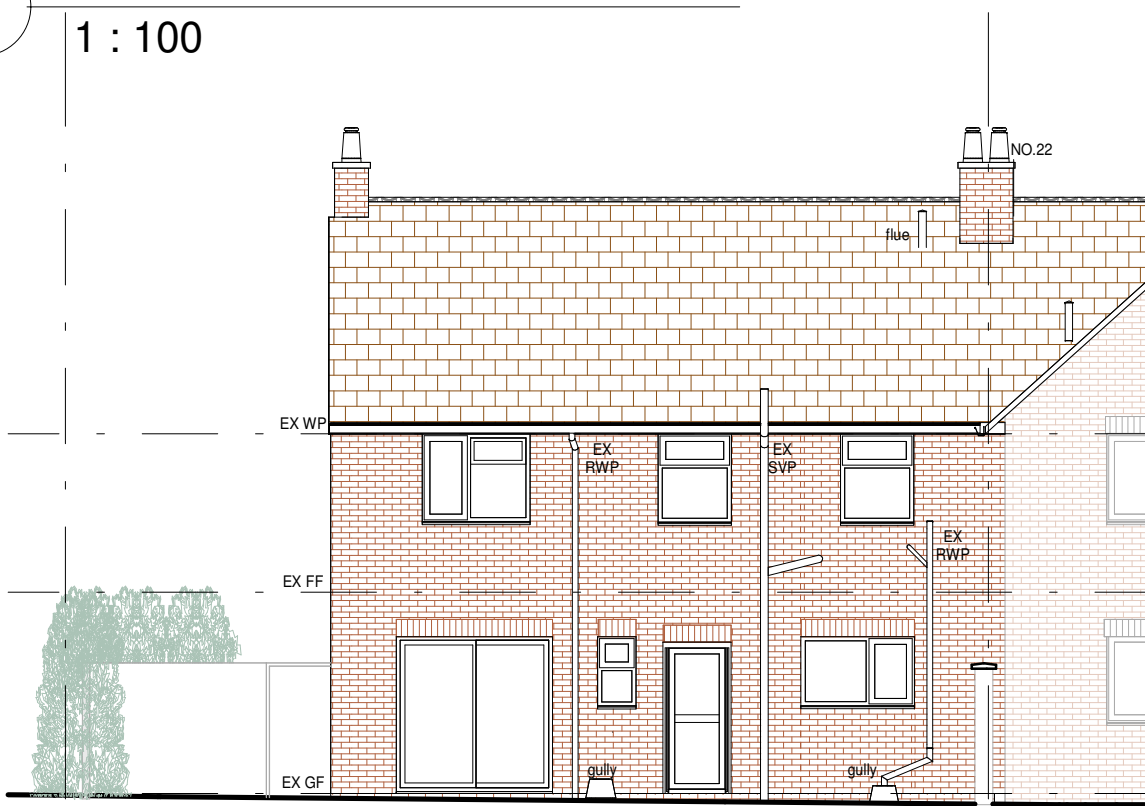
5 Existing West Elevation 1 : 100
