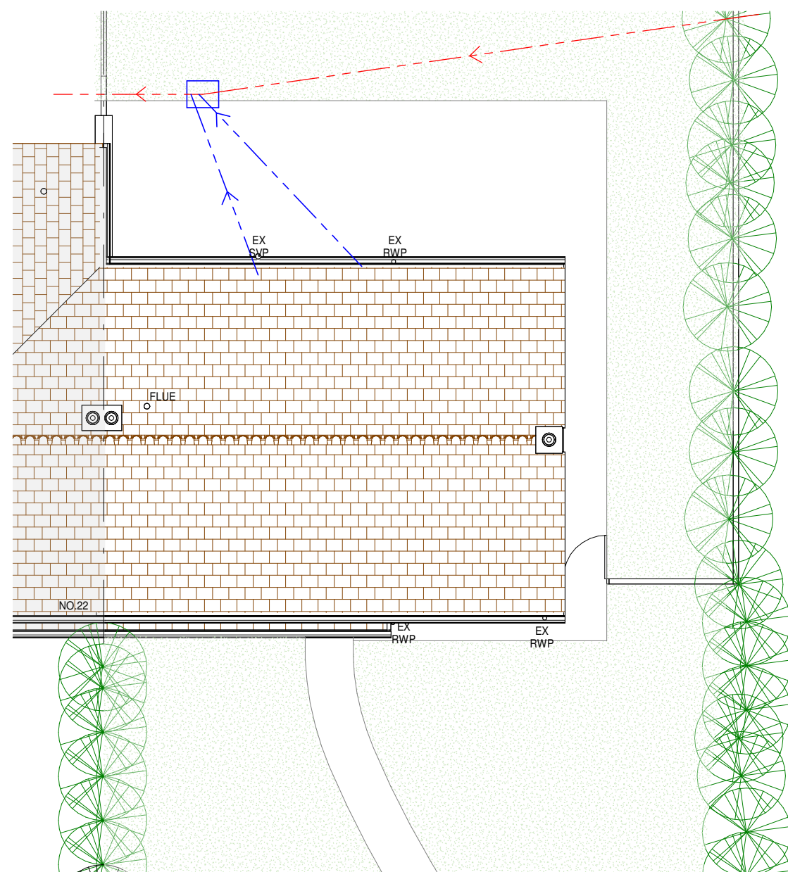
2 Existing Roof Plan 1 : 100
