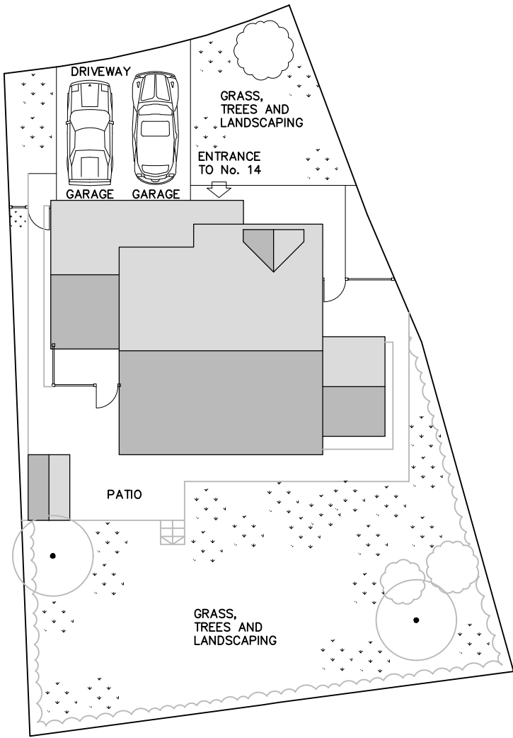
EXISTING SITE AND ROOF PLAN 1:200
