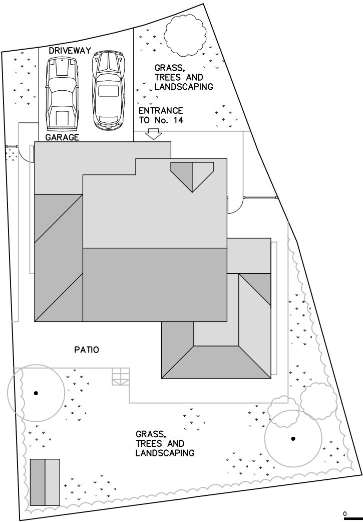
PROPOSED SITE AND ROOF PLAN 1:200
