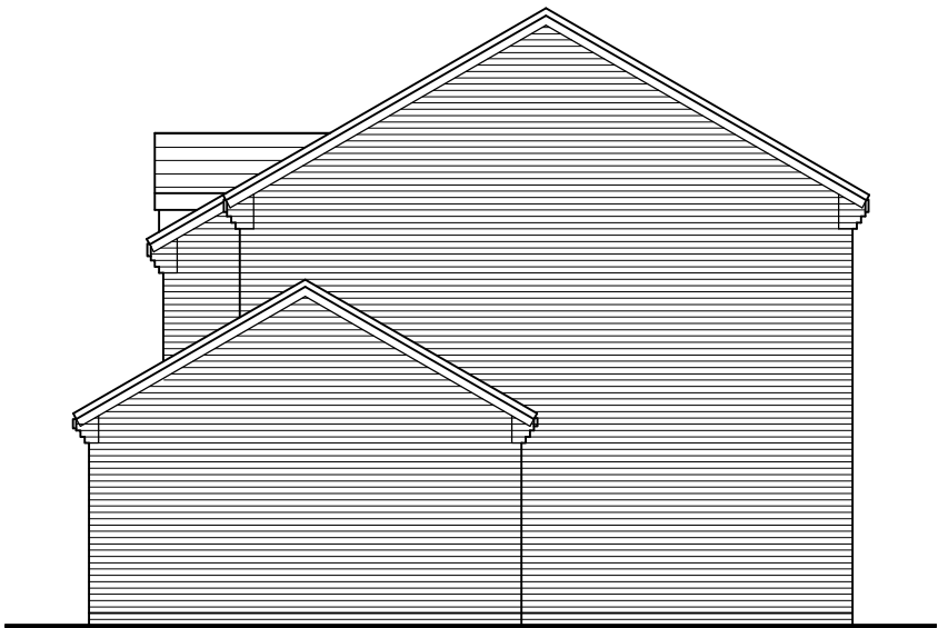
EXISTING WEST SIDE ELEVATION
