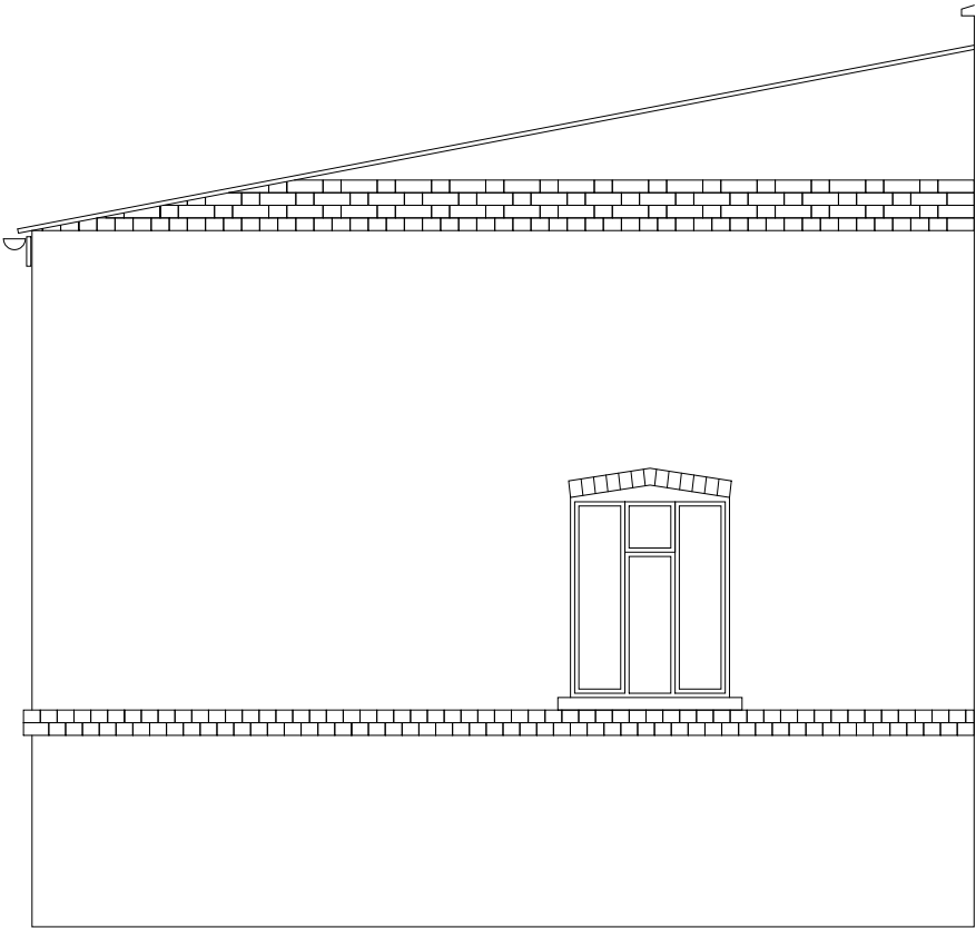
Existing West Elevation
