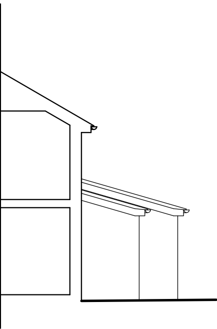
Side Elevation/Section @ 1/100
