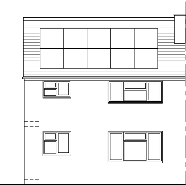
Rear Elevation (unchanged) @ 1/100
