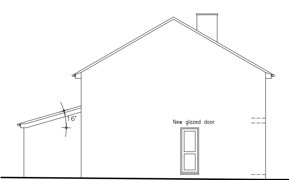
Side Elevation @ 1/100
