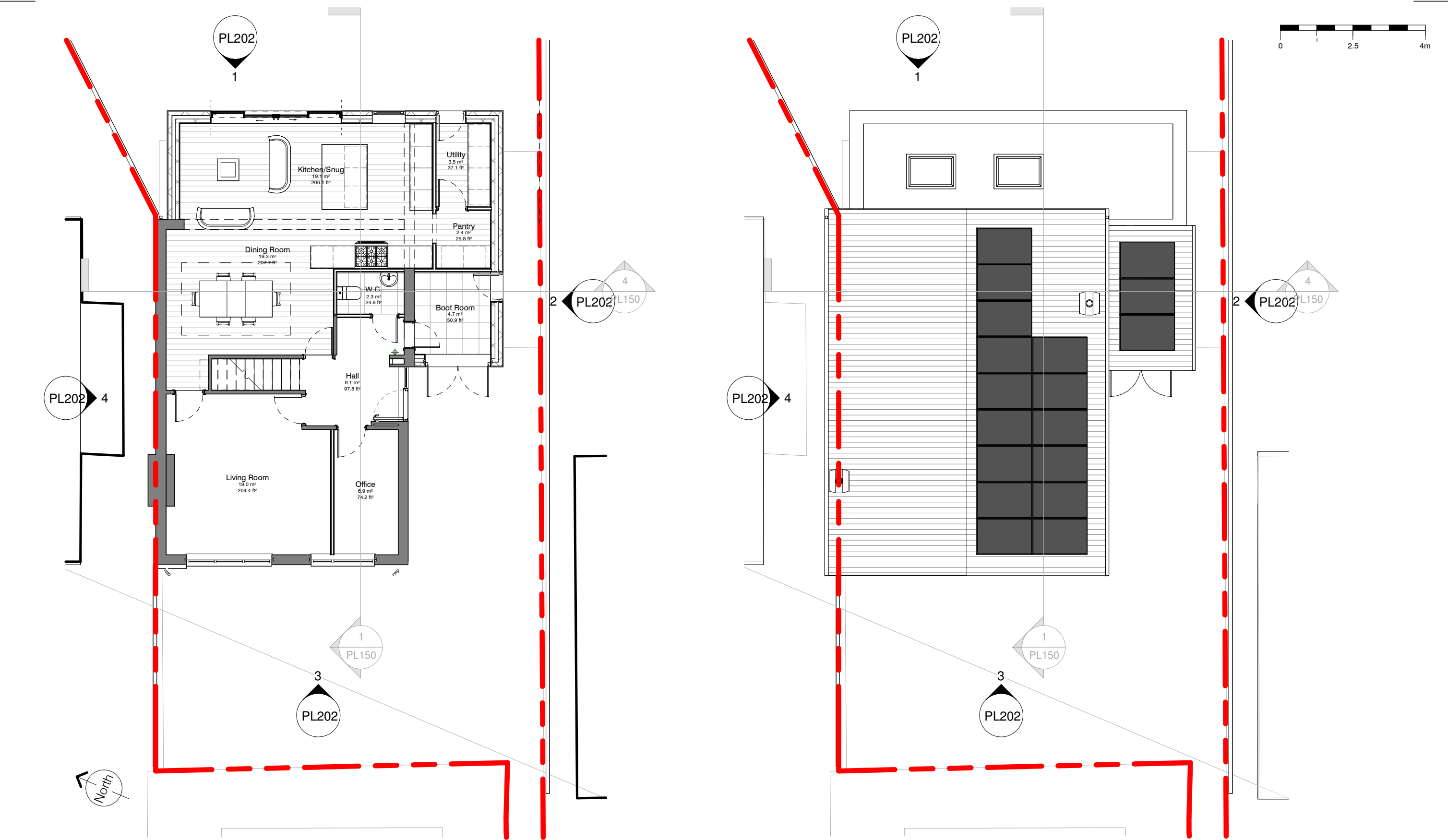
1 GROUND - Proposed C 1 : 100 @A3
