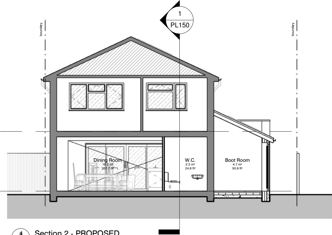
4 Section 2 - PROPOSED 1 : 100 @A3
