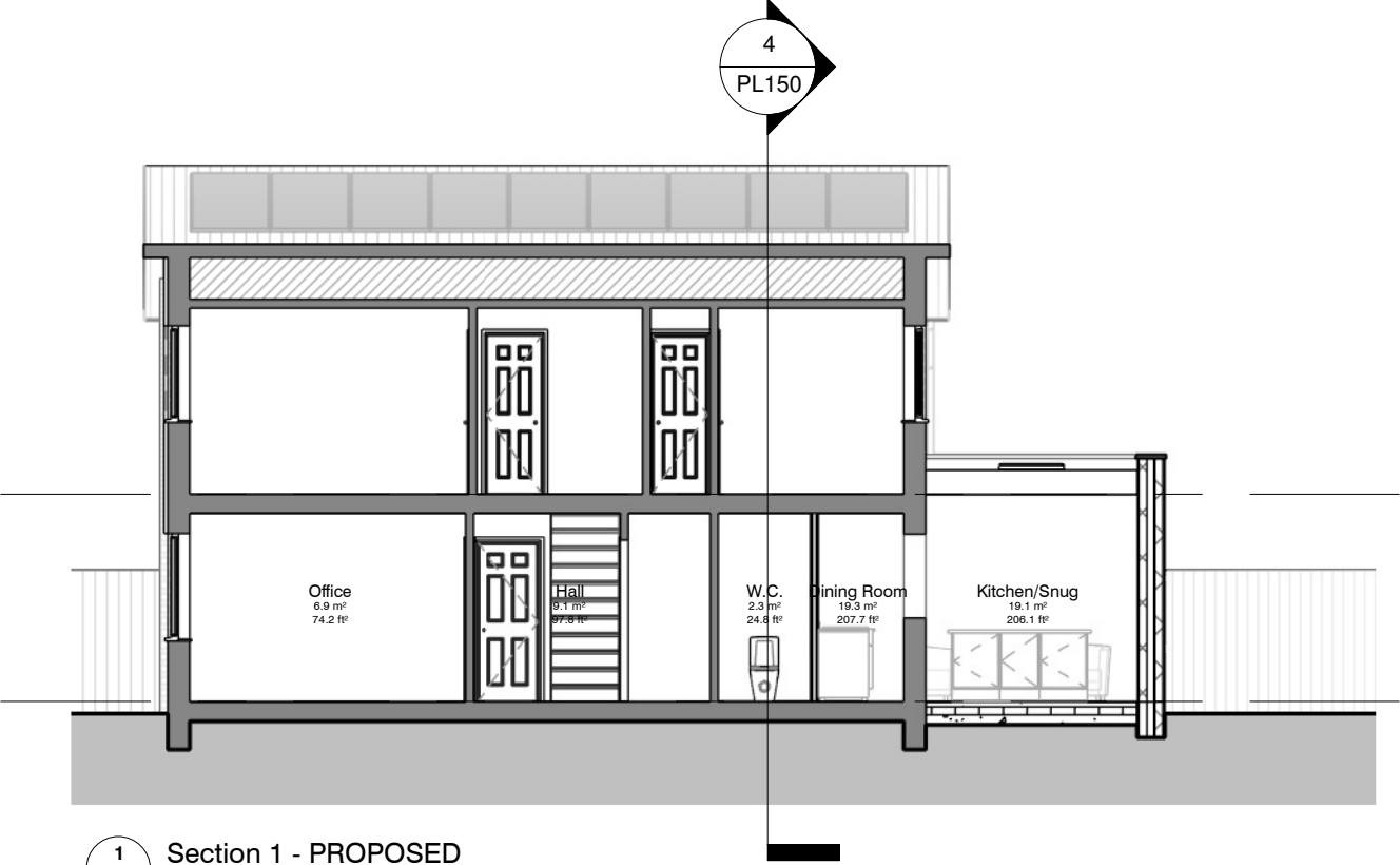
1 Section 1 - PROPOSED 1 : 100 @A3
