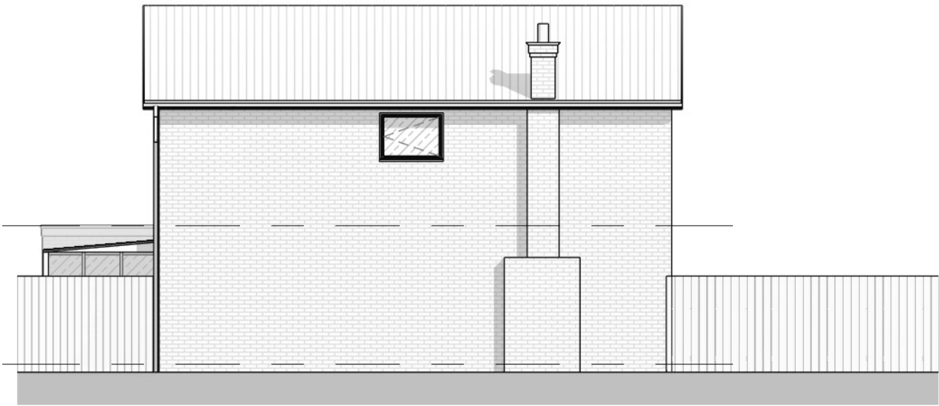
4 EXISTING - Boundary Elevation 1 : 100 @A3
