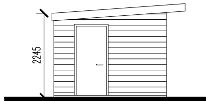
South Elevation
