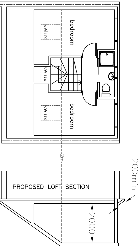
PROPOSED LOFT
