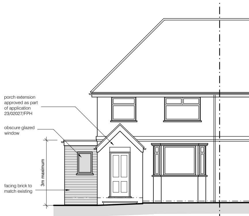
Front Elevation
