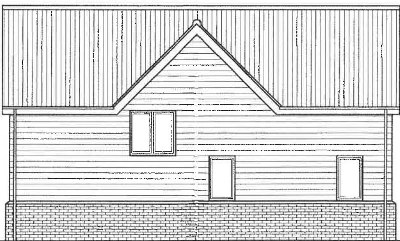
West Elevation
