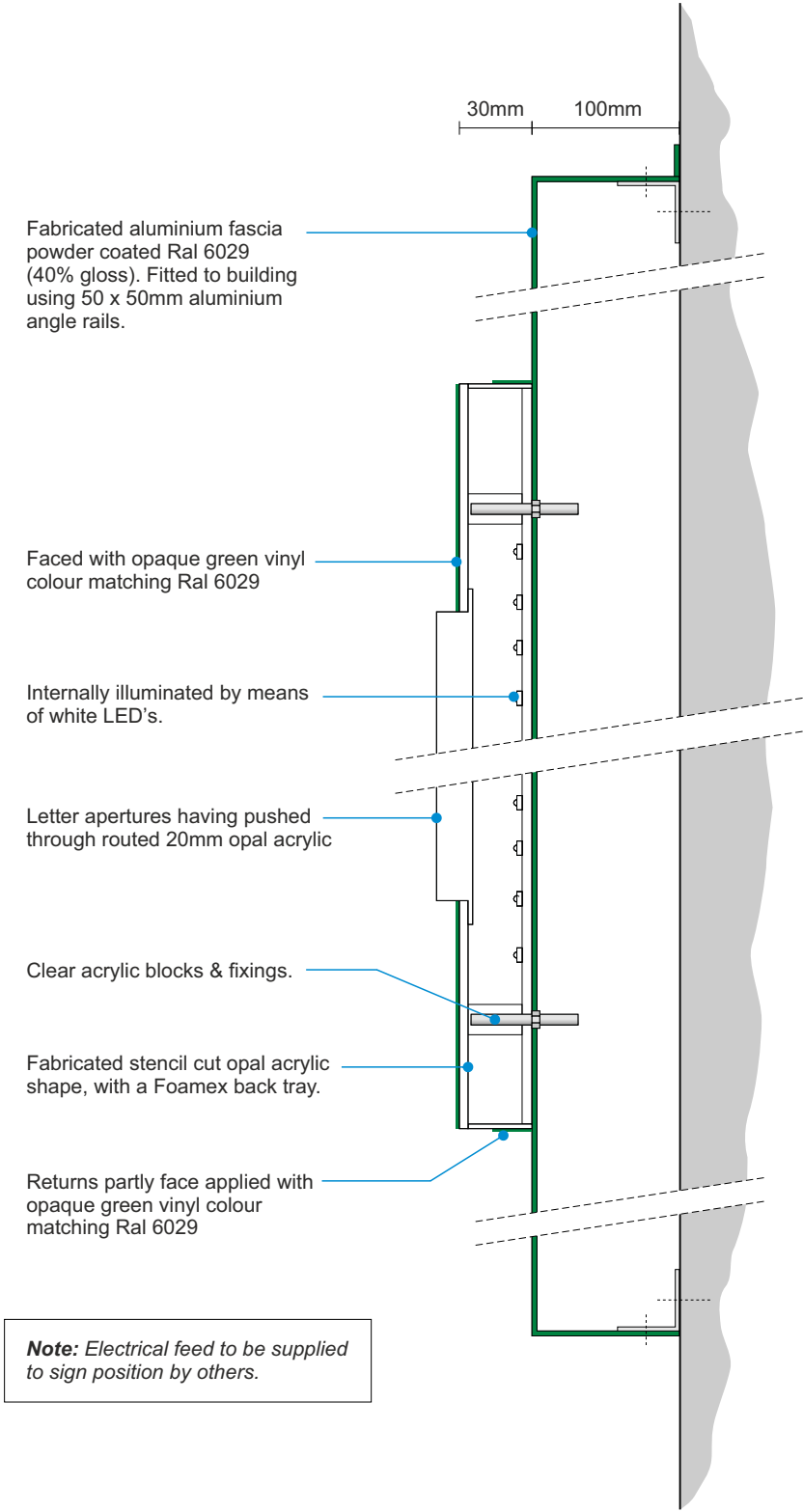
Logo section Scale 1:5
