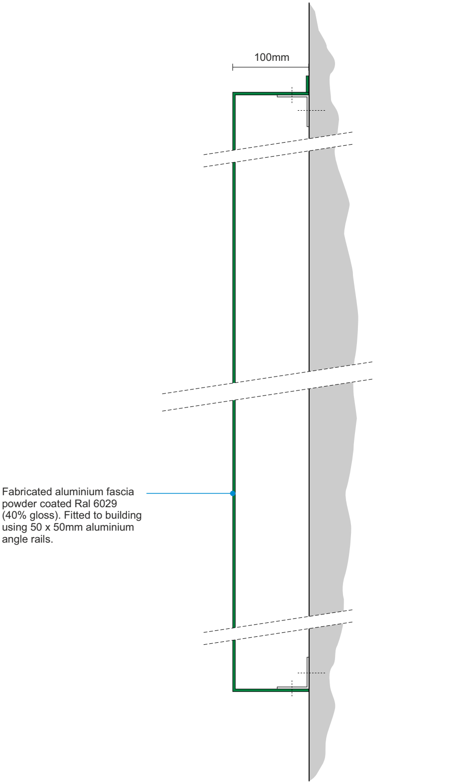
Non illuminated fascia section Scale 1:5
