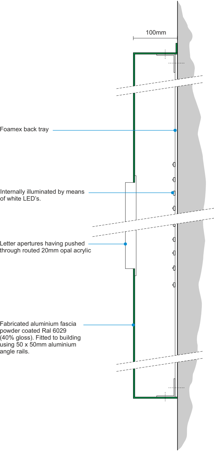
Sub text section Scale 1:5
