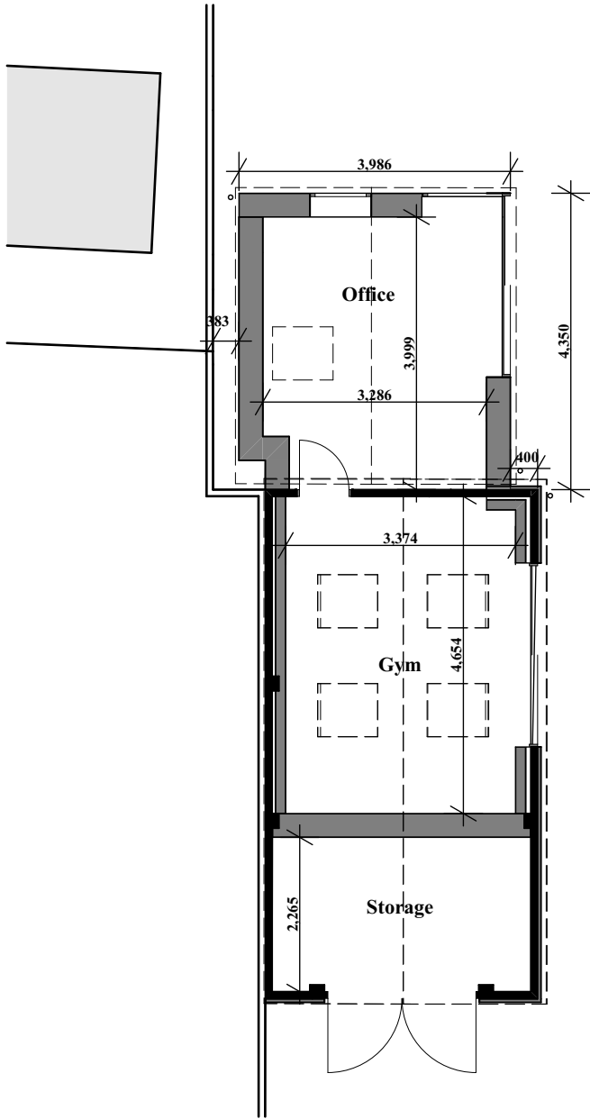
1:100 Proposed Ground Floor Plan
