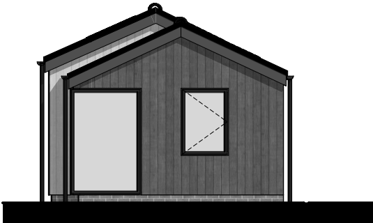
1:100 Proposed South West Elevation
