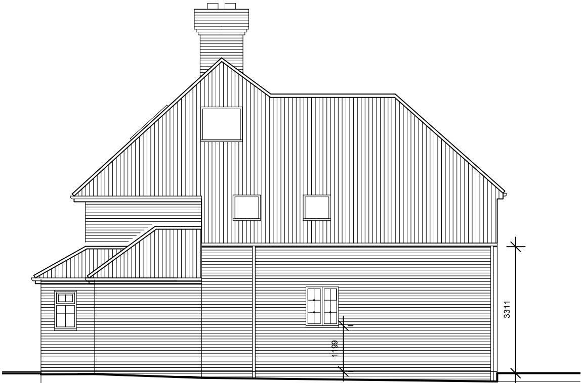
EXISTING SIDE(WEST) ELEVATION
