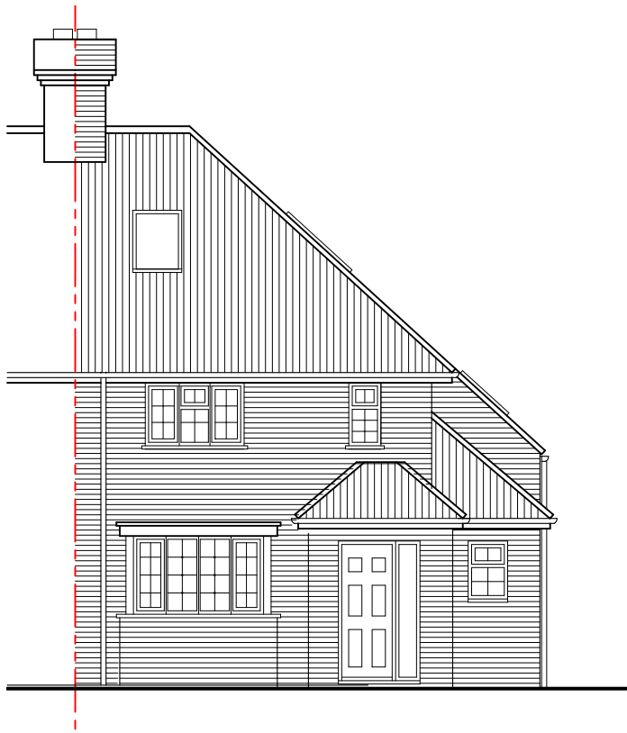
EXISTING FRONT (NORTH) ELEVATION
