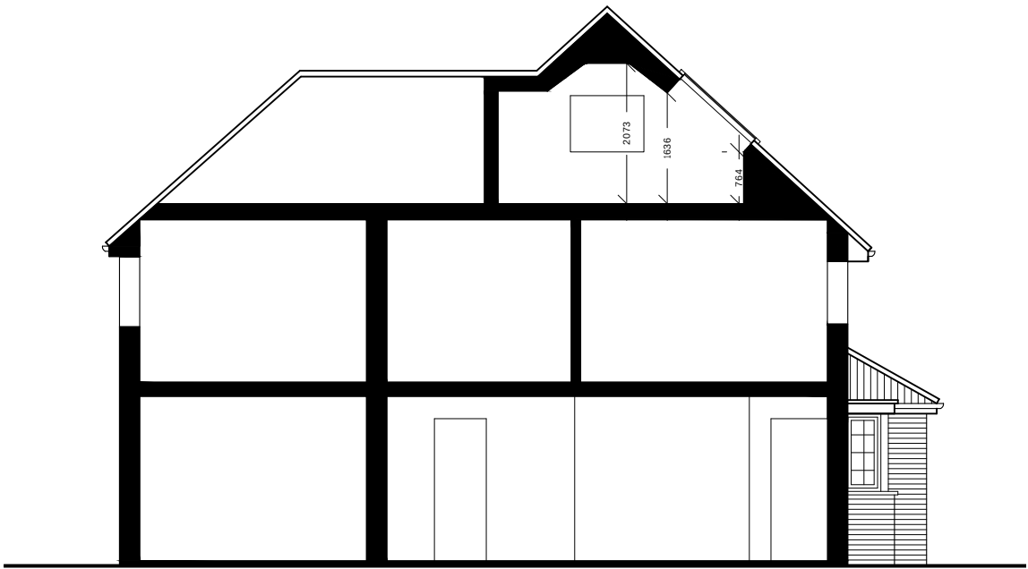
EXISTING SIDE (EAST) ELEVATION / SECTION
