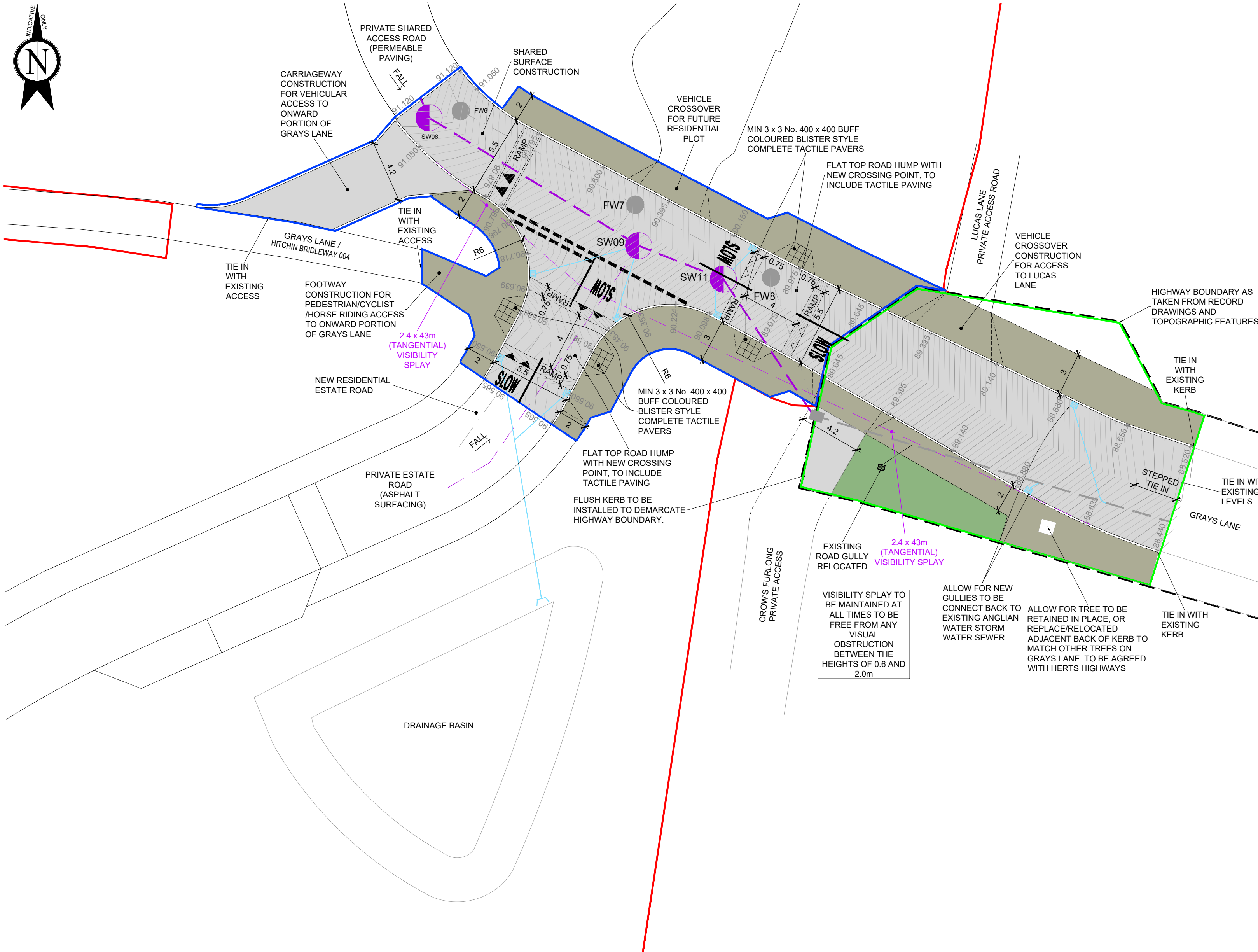
PROPOSED S278 WORKS 1:200
