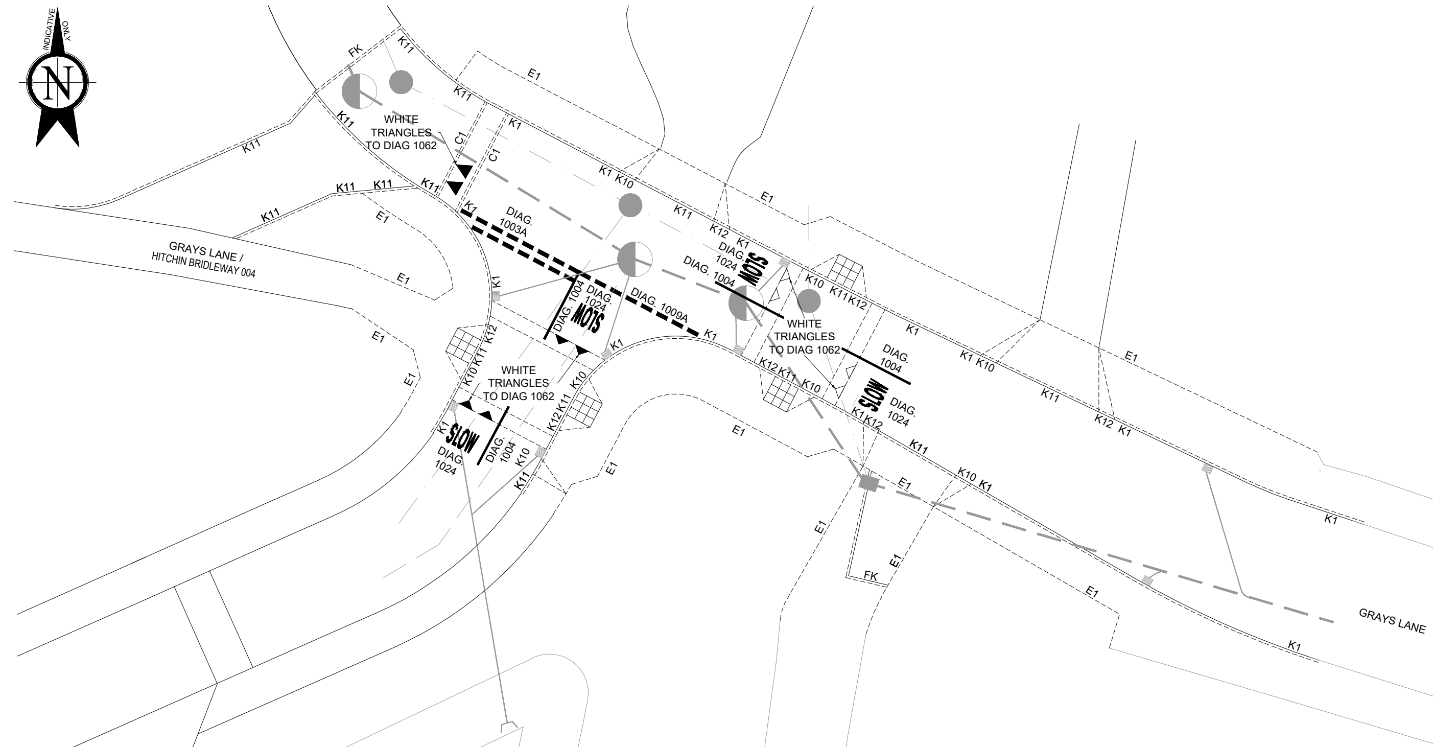
KERB AND ROAD MARKING LAYOUT 1:200
