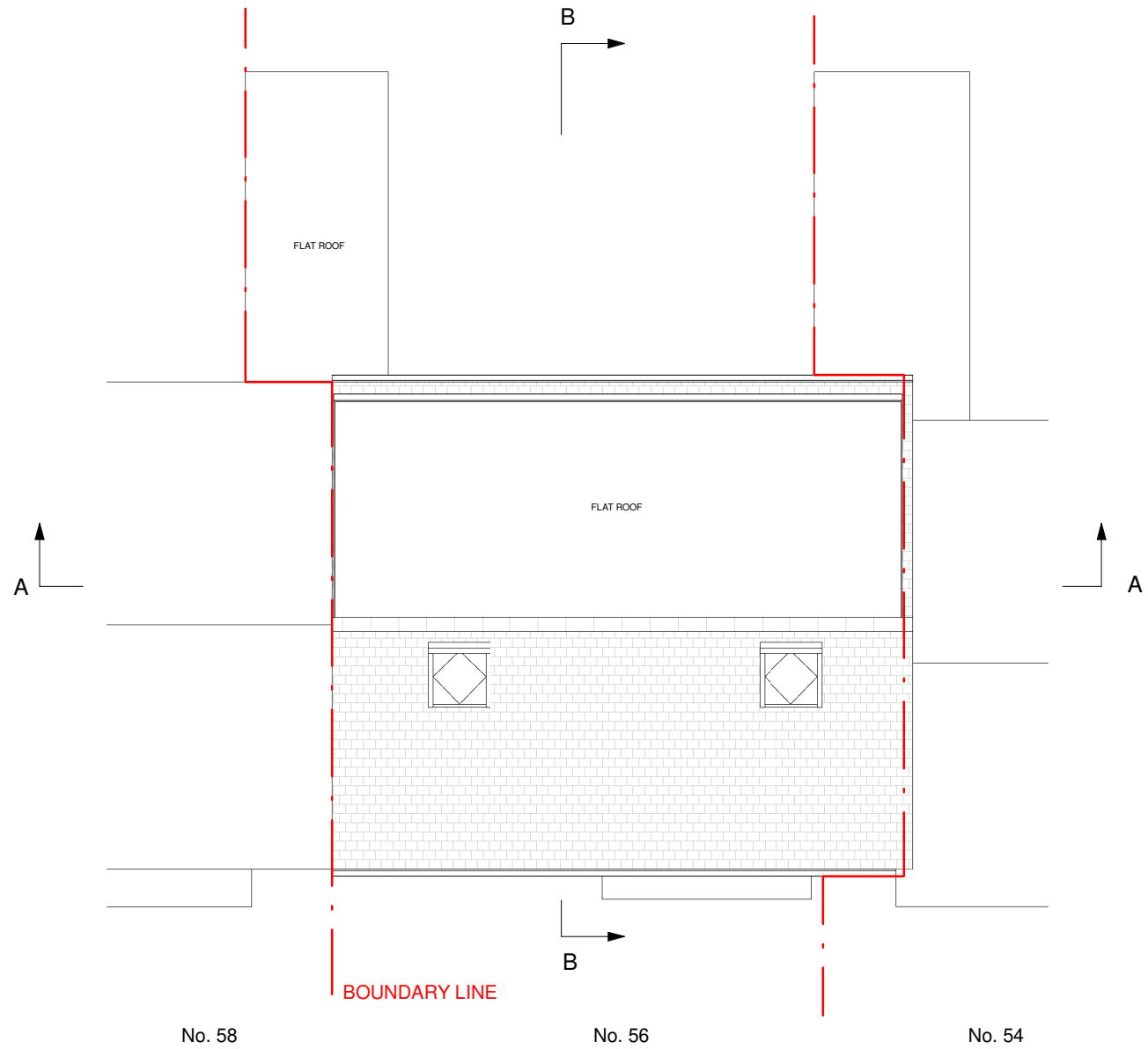
PROPOSED ROOF PLAN 1:100 @ A3
