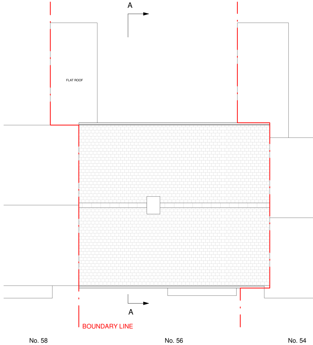
EXISTING ROOF PLAN 1:100 @ A3
