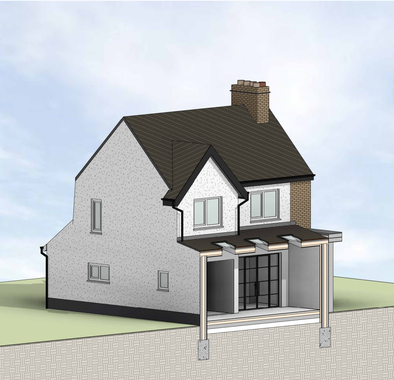
3D SECTION
