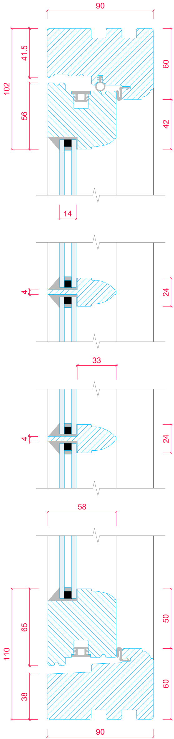
CASEMENT CROSS SECTION 'A-A' (SCALE 1:2)
