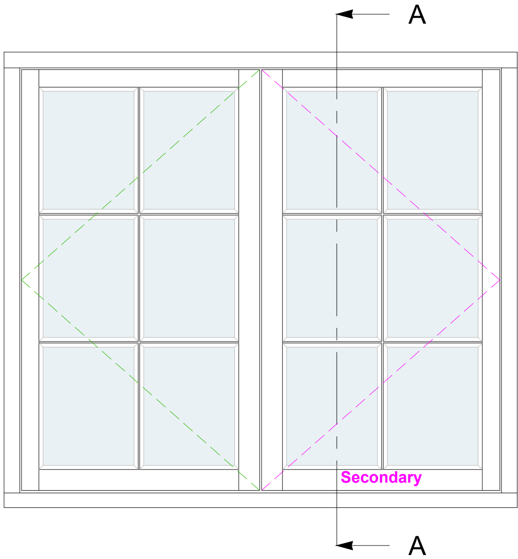
TYPICAL CASEMENT LAYOUT (SCALE 1:10)
