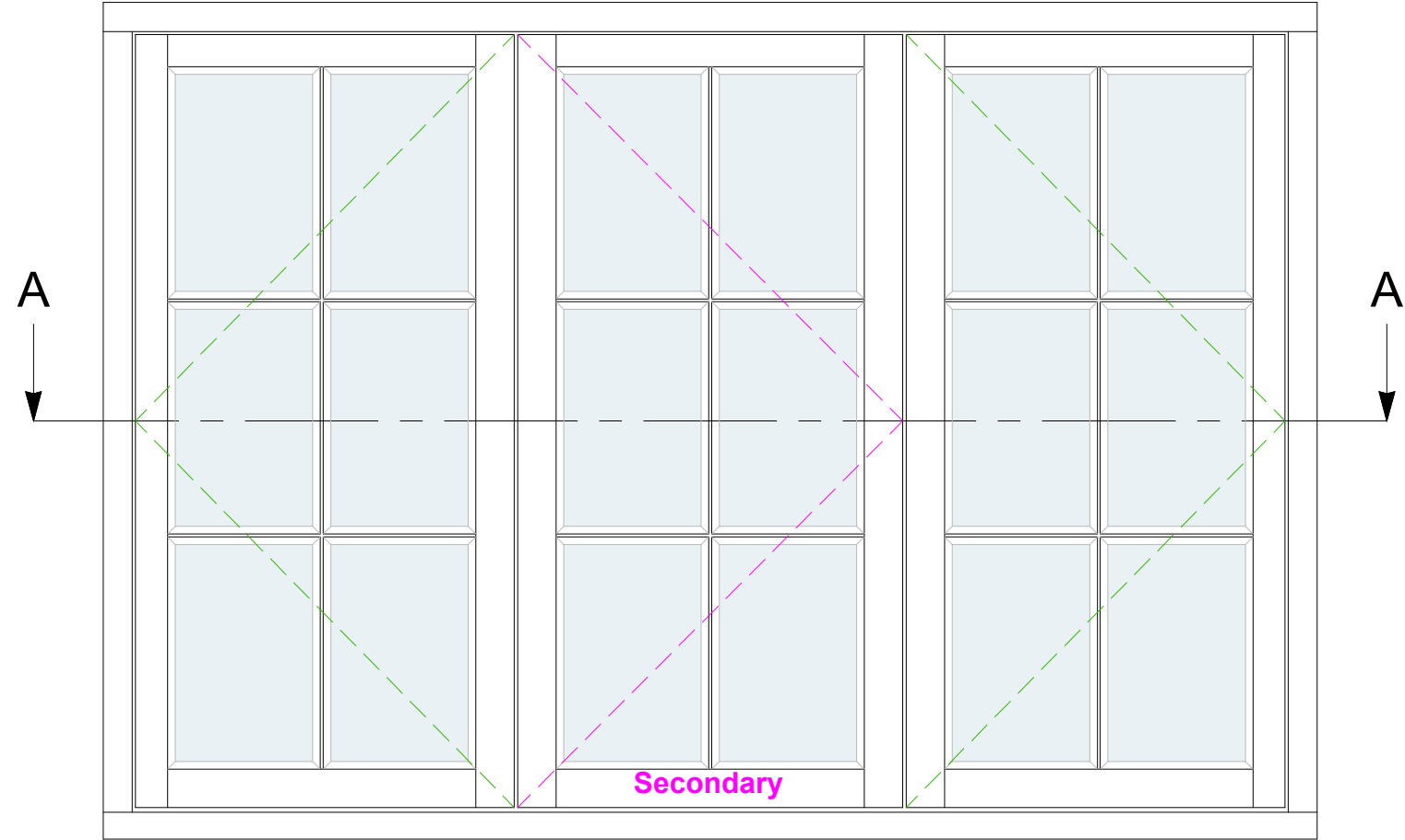
TYPICAL CASEMENT LAYOUT (SCALE 1:10)
