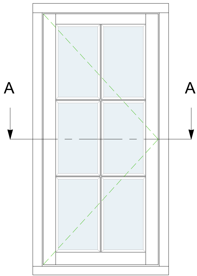
TYPICAL CASEMENT LAYOUT (SCALE 1:10)
