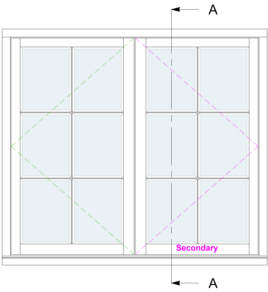
TYPICAL CASEMENT LAYOUT with 25mm Cill Extension (115mm) (SCALE 1:10)
