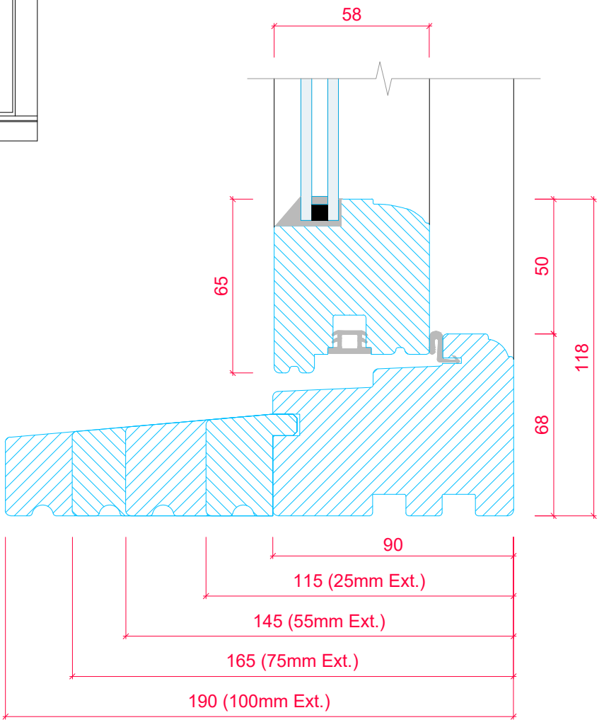
CASEMENT CROSS SECTION 'A-A' (SCALE 1:2)
