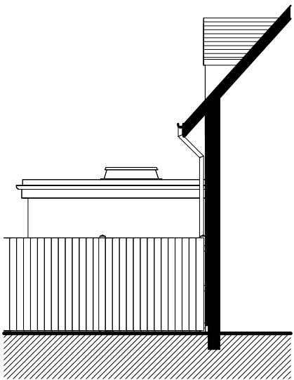
Proposed NorthWest Elevation 1 : 100
