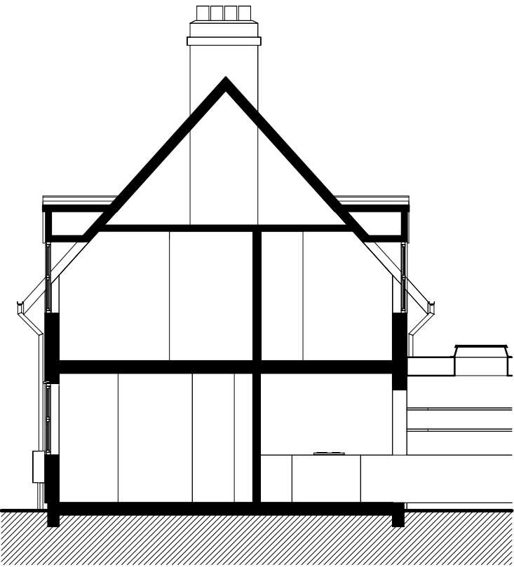
Proposed Section 1 : 100
