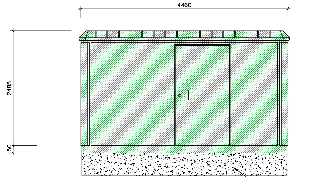
Front Elevation
