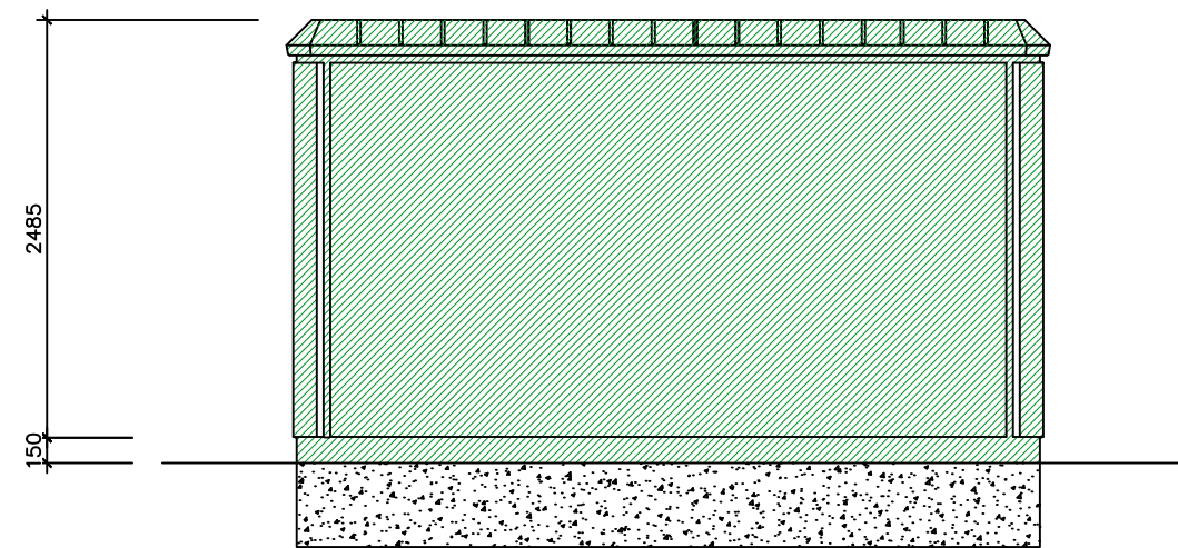
Rear Elevation
