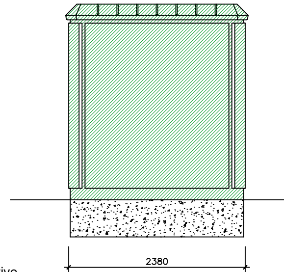
LEFT ELEVATION
