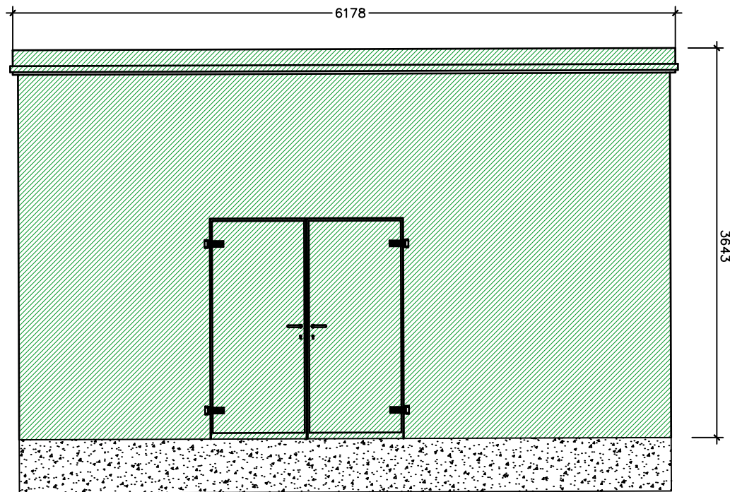
Front Elevation
