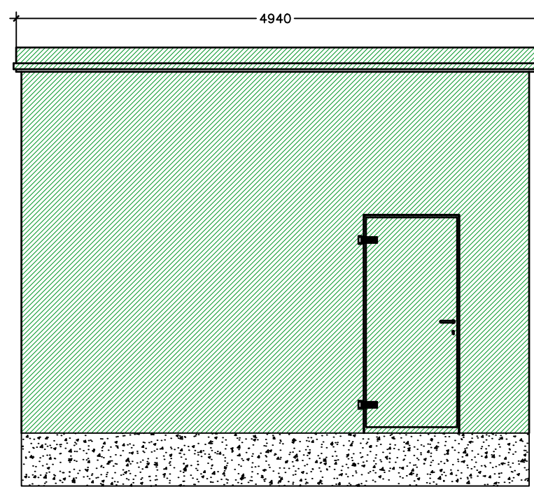
Left Elevation
