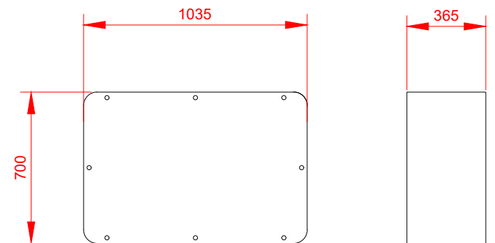
String Inverter (1:25)
