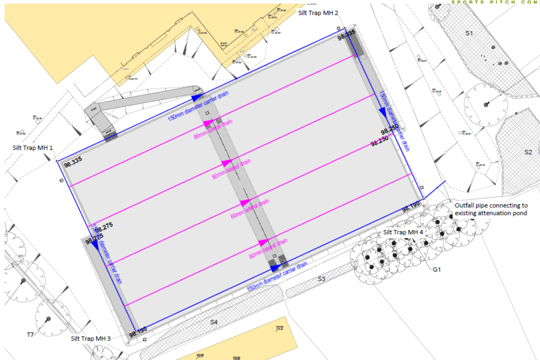
Figure 13 - Drainage Layout
