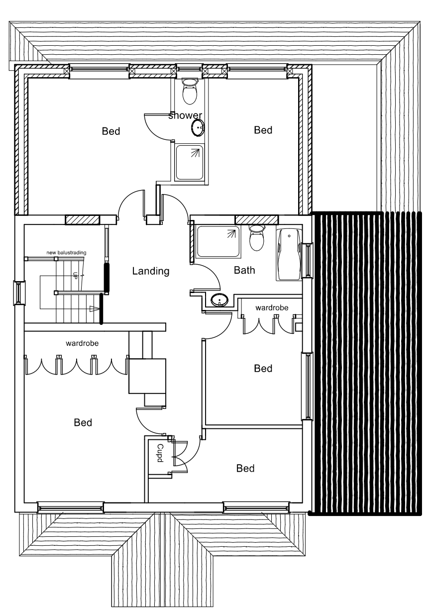
FIRST FLOOR (PROPOSED)
