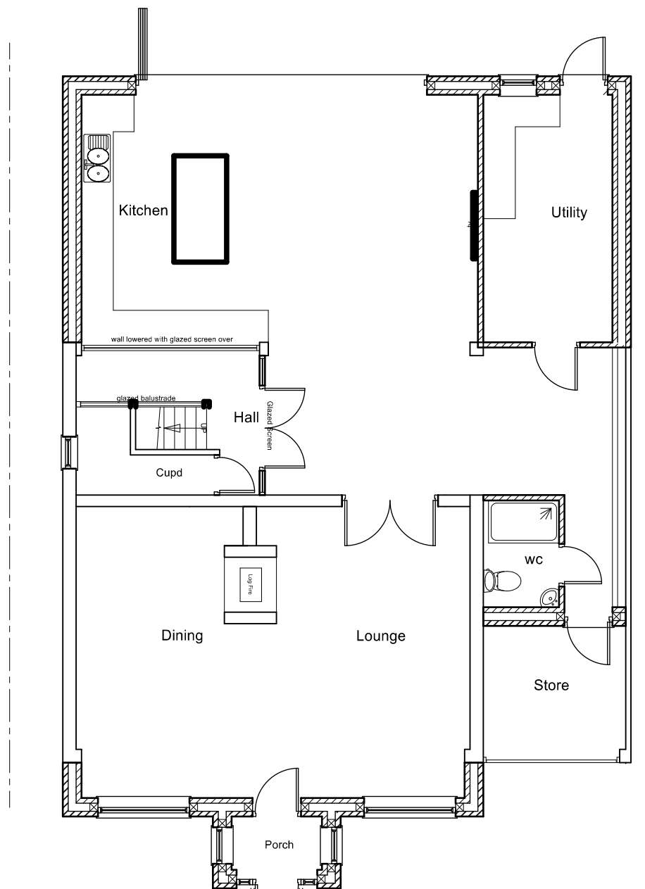
GROUND FLOOR (PROPOSED)
