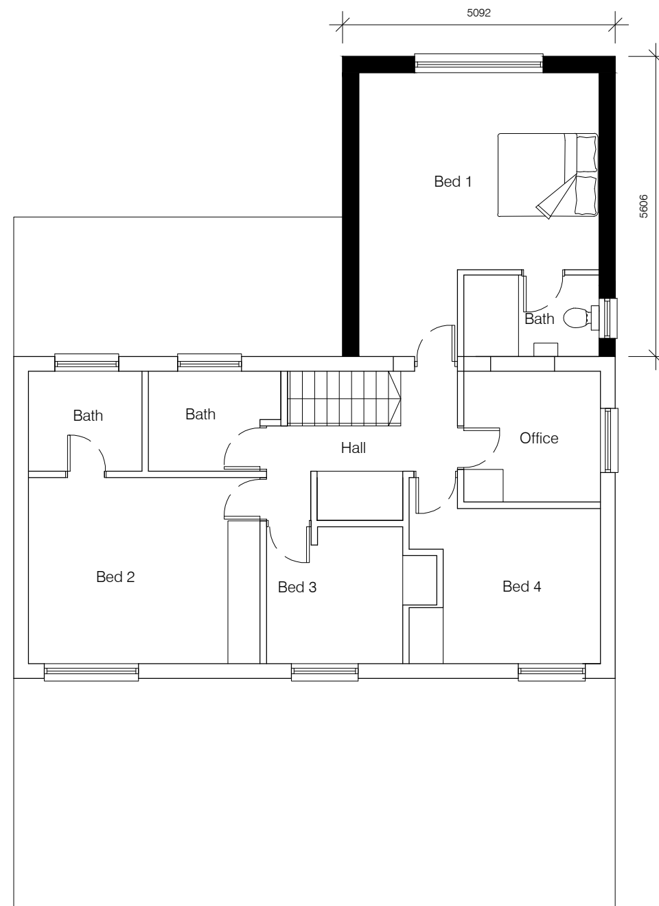
Proposed First Plan 1:100
