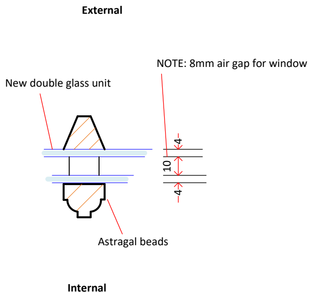
PROPOSED REAR GF ASTRAGALS
