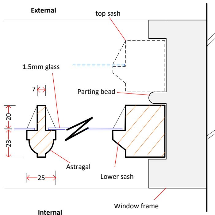
EXISTING SLIDING SASH
