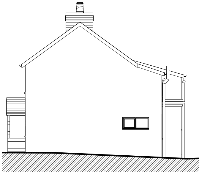
Existing South Elevation 1 : 100
