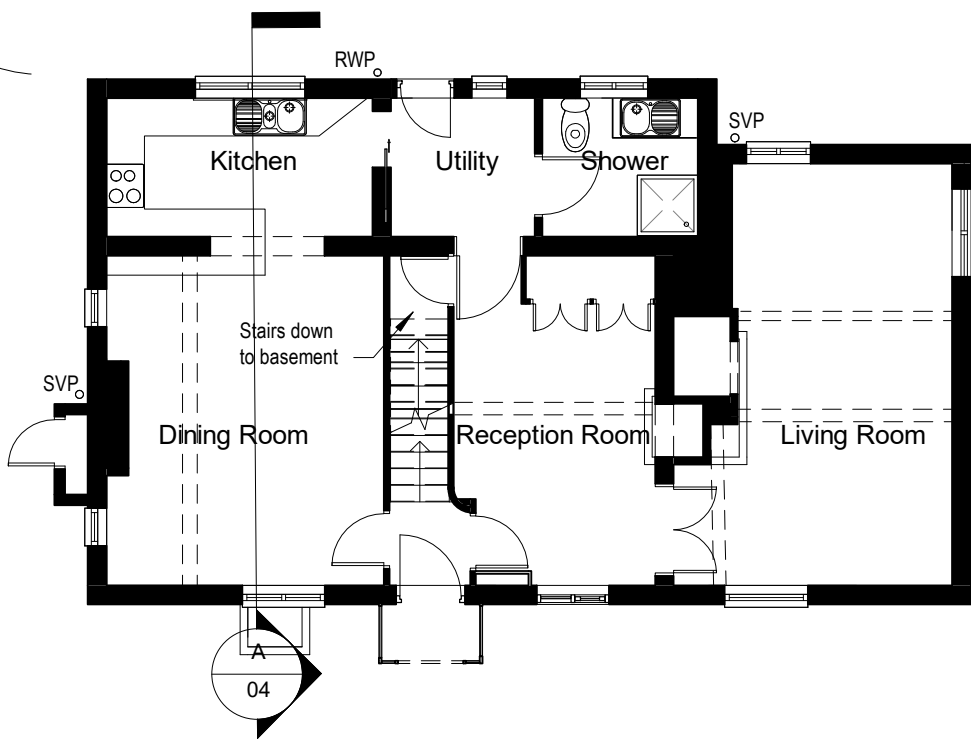
Existing Ground Floor 1 : 100
