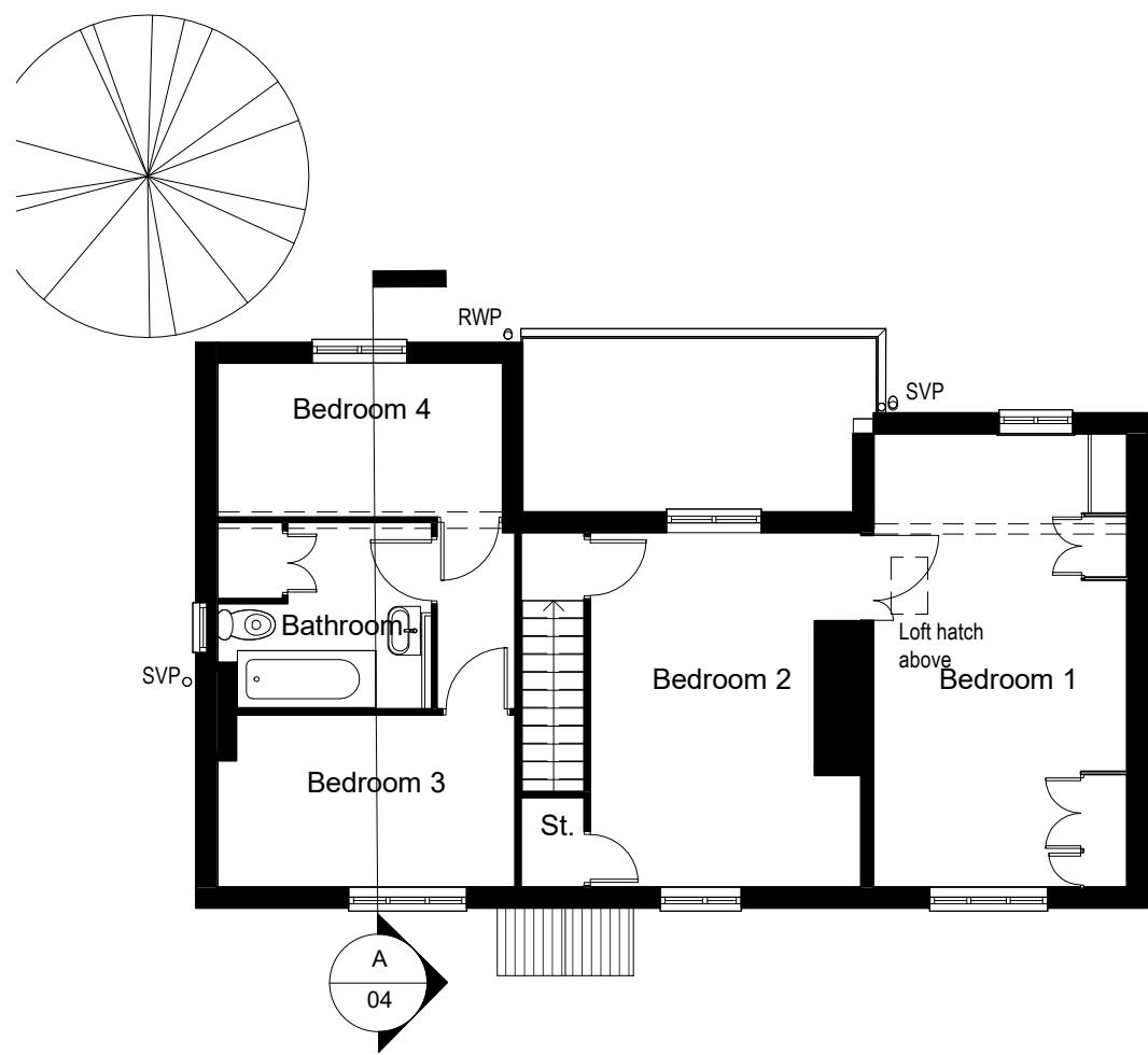
Existing First Floor 1 : 100
