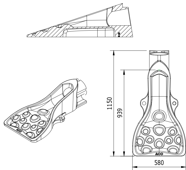
ACO SWALE INLET FOR 1500 PIPES
