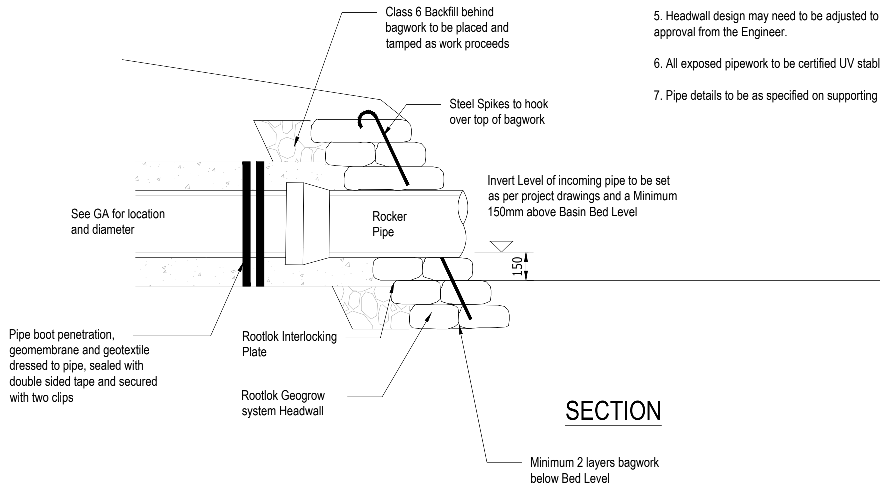
BAGWORK HEADWALL FOR 225mm - 375mm PIPES
