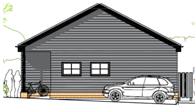
Figure 11 - Proposed right side elevation
