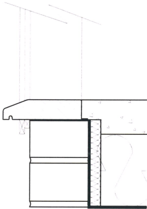
Door threshold detail for Part M.
