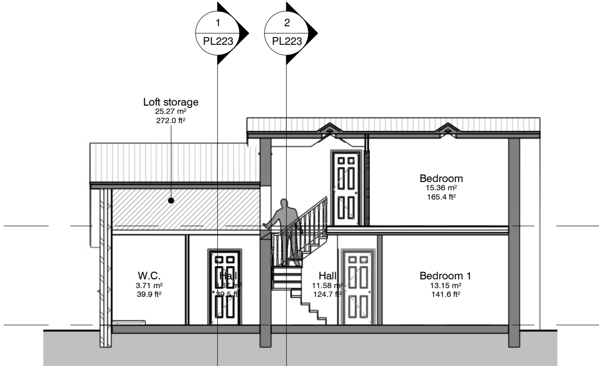
3 Section 3 - Proposed 1 : 100 @A3
