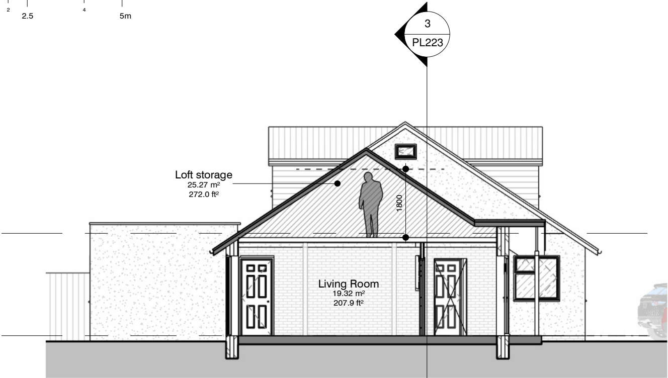
1 Section 1 - Proposed 1 : 100 @A3
