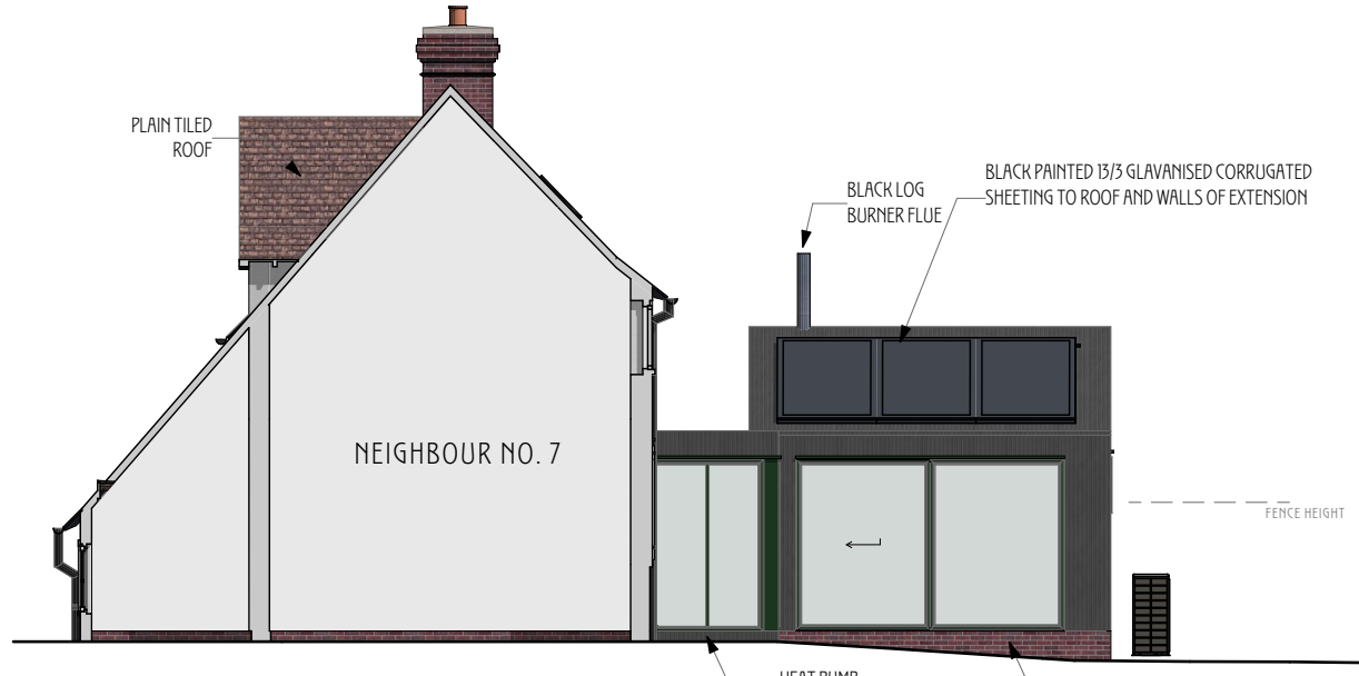
NEIGHBOUR NO. 7 PROPOSED NORTH WEST ELEVATION
