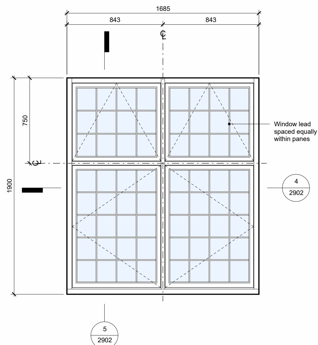
3 Window Type B - Elevation 1 : 20
