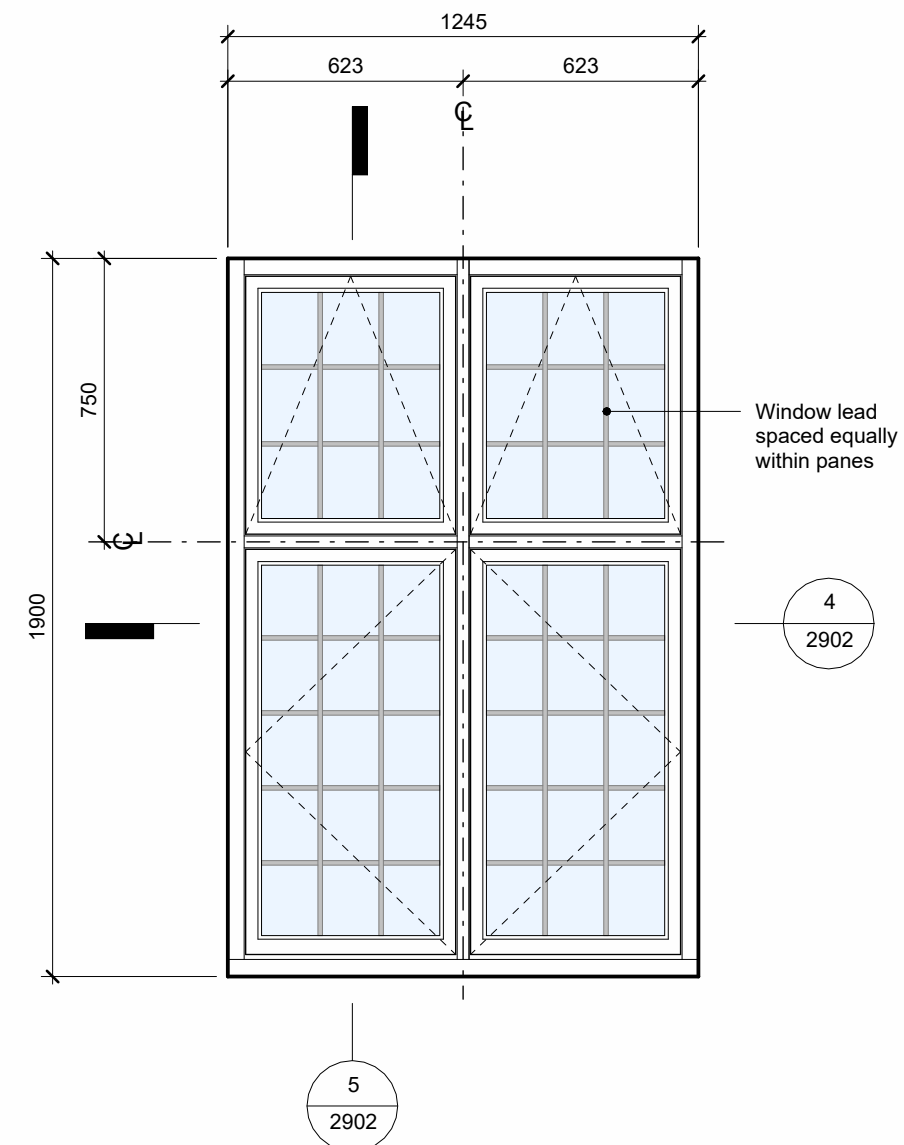
2 Window Type A - Elevation
