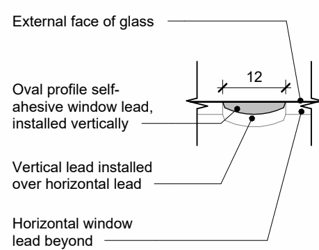
6 Plan Detail - Glazing Bar 1:1
