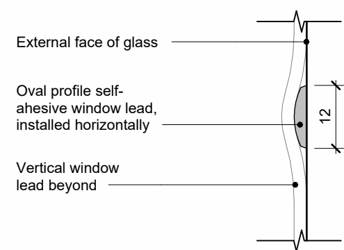
7 Section Detail - Glazing Bar 1:1
