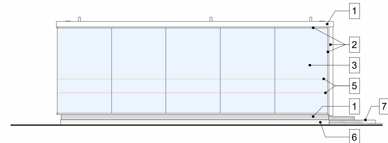
2 Southwest Elevation 1 : 100
