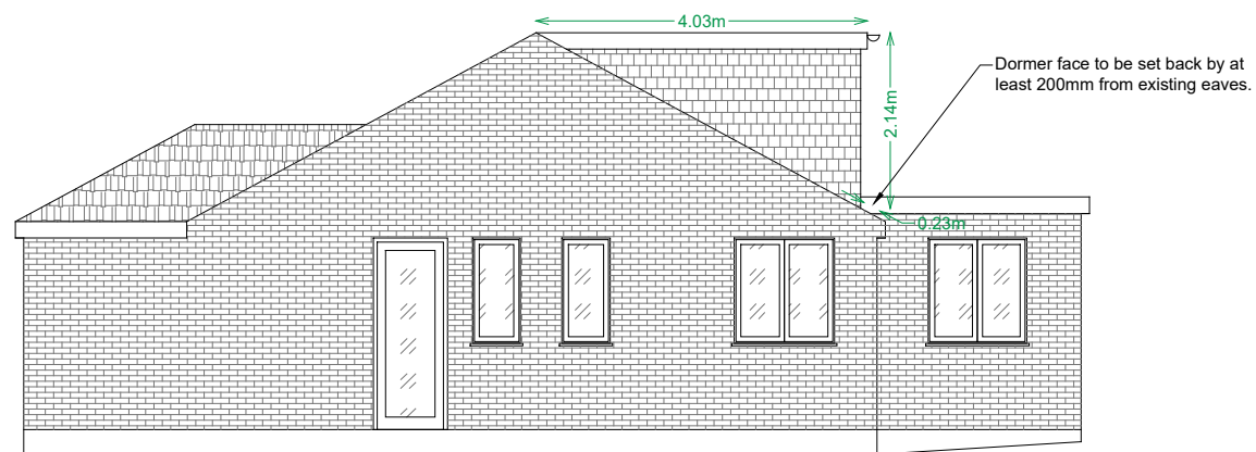
PROPOSED SIDE ELEVATION B
