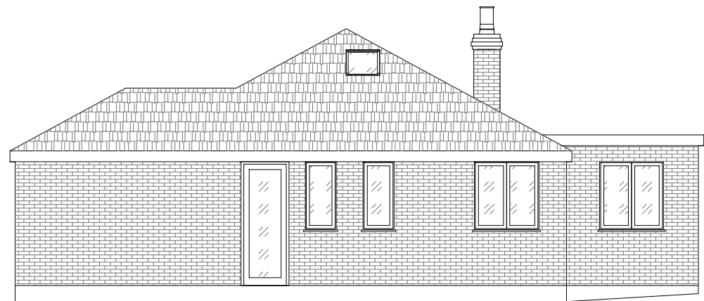
EXISTING SIDE ELEVATION B
