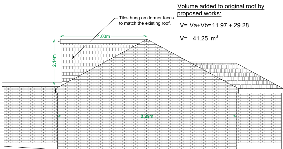
PROPOSED SIDE ELEVATION A
