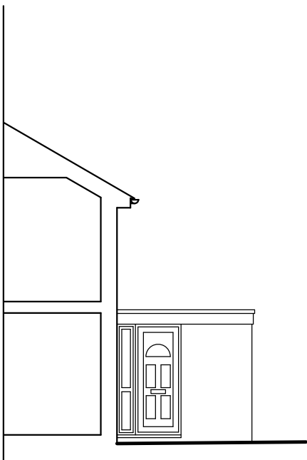
Side Elevation/Section @ 1/100
