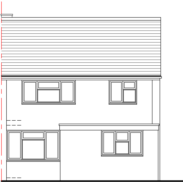
Front Elevation @ 1/100
