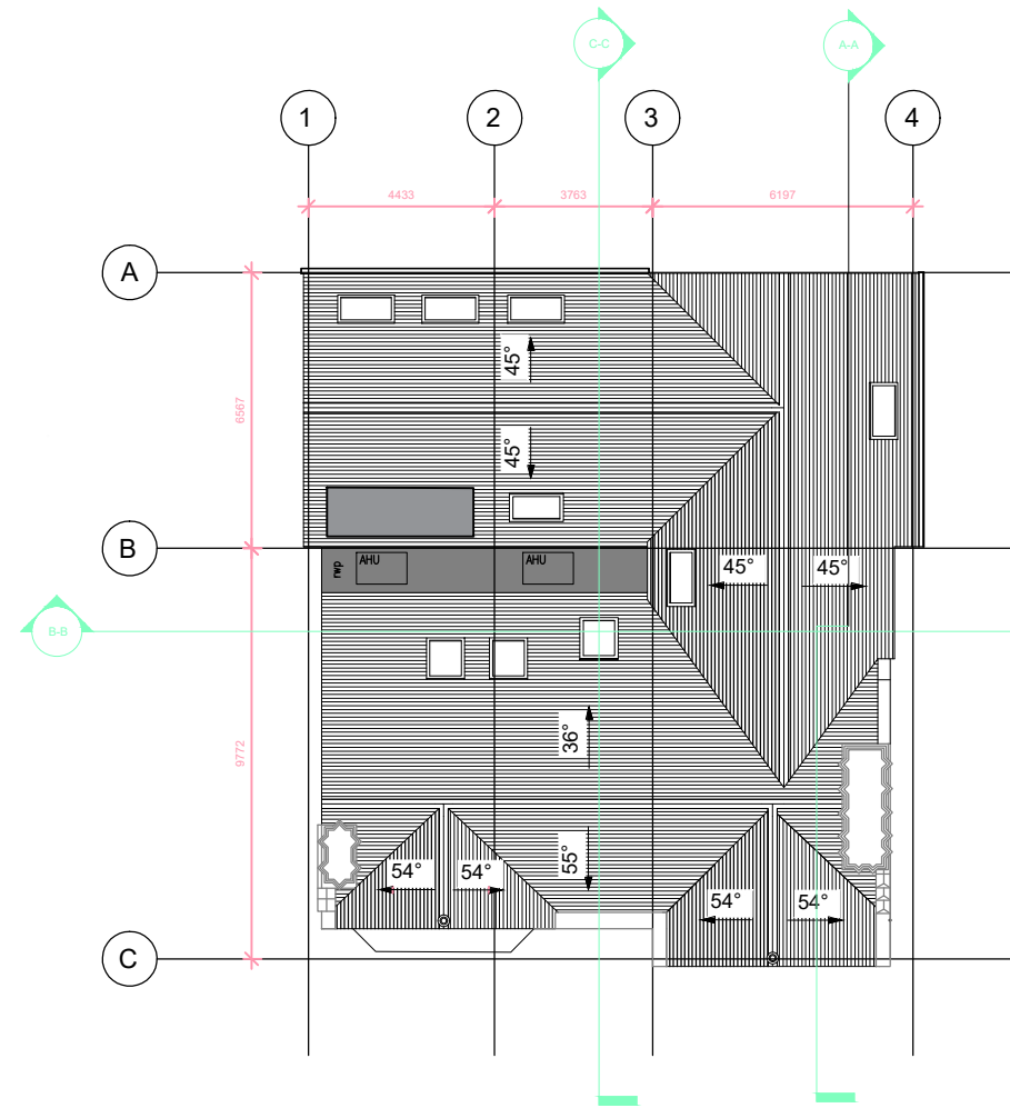
Roof
