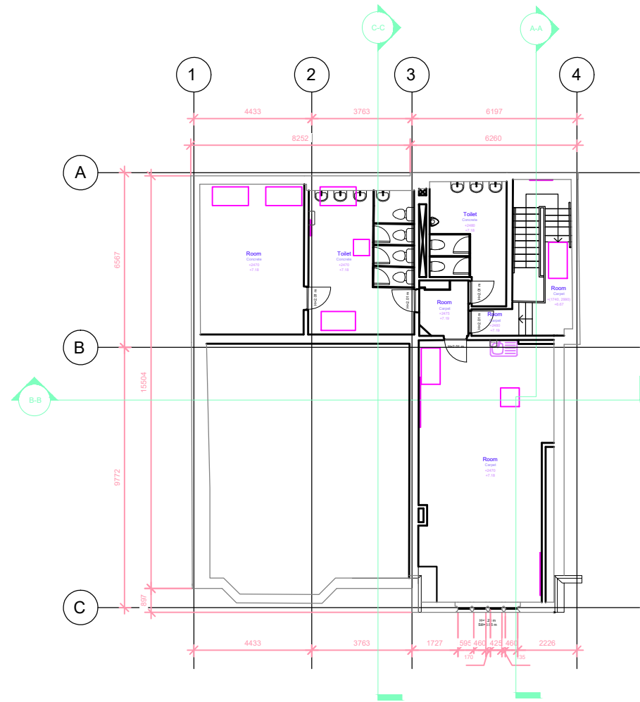
Second Floor
