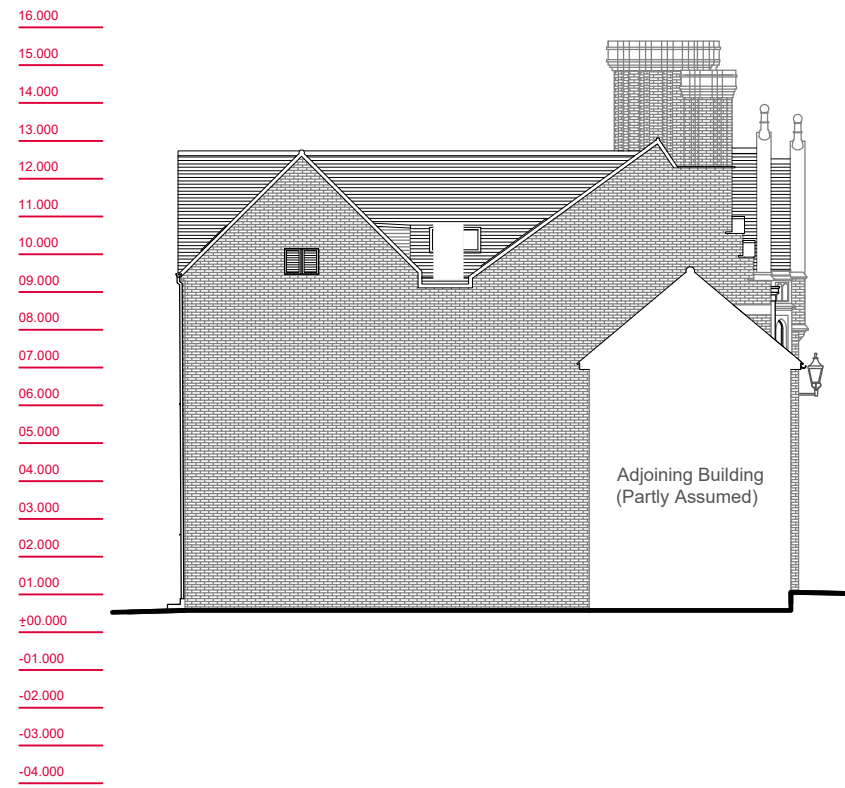
Left Elevation
