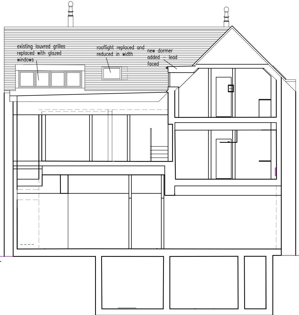
Section B-B
