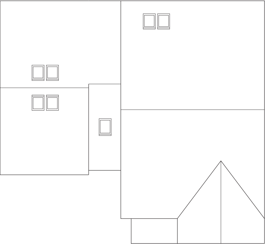
Roof Plan
