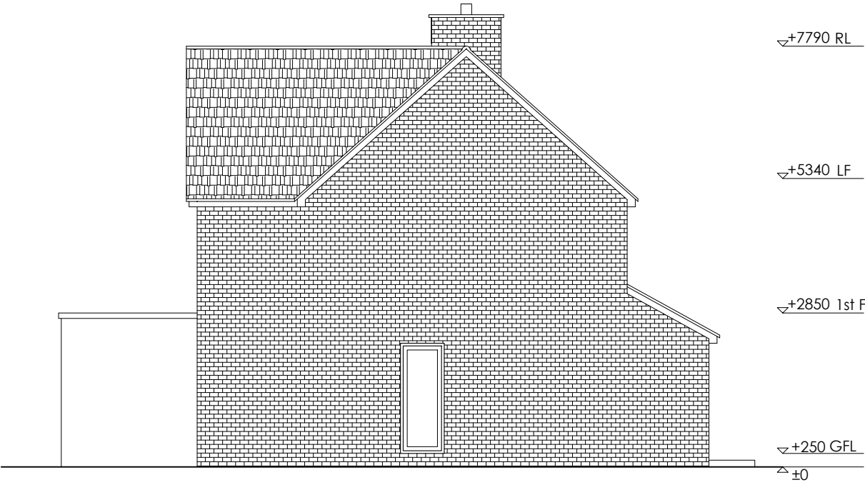
03 A-303 EXISTING LEFT ELEVATION SCALE- 1:100@A3
