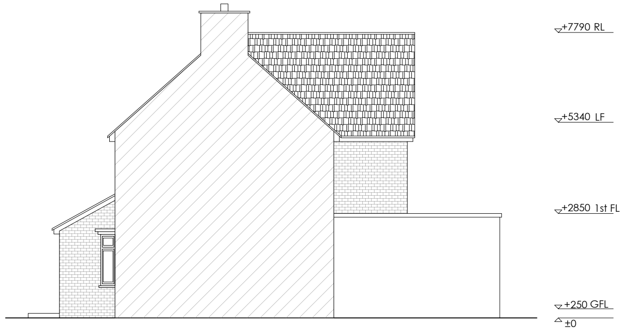
02 A-305 PROPOSED RIGHT ELEVATION SCALE- 1:100@A3
