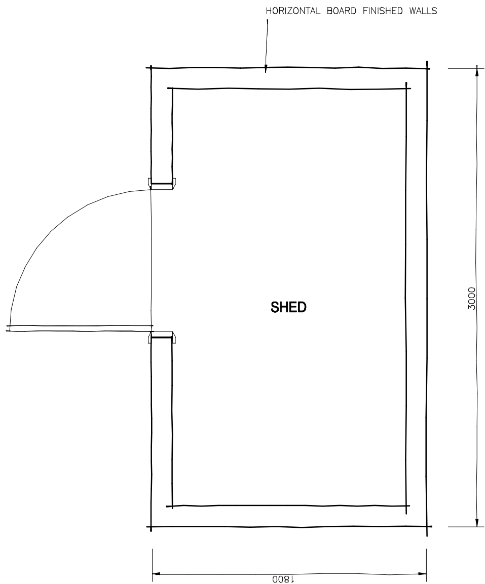
FLOOR PLAN
