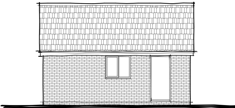
REAR ELEVATION (SOUTH)
