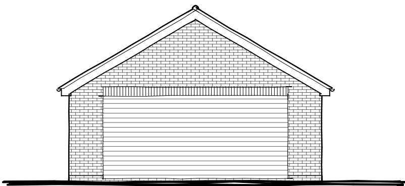
SIDE ELEVATION (EAST)
