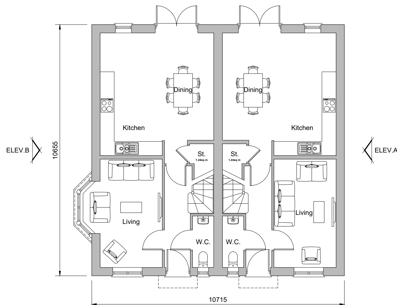
Ground Floor Plan Plots 47-48 Plots 16-17 (Handed)
